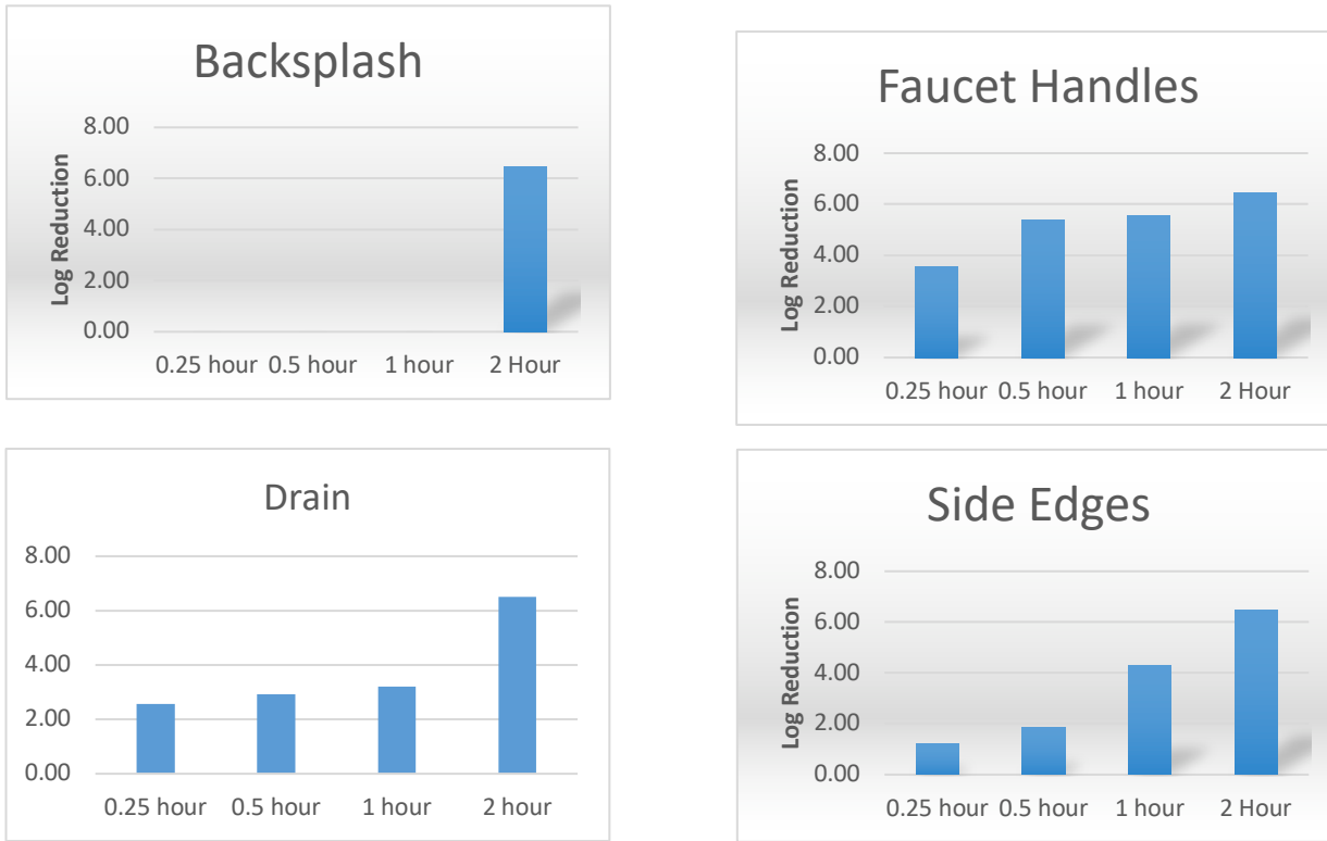
Figure 5: UV Reduction of MRSA after 2 Hours
