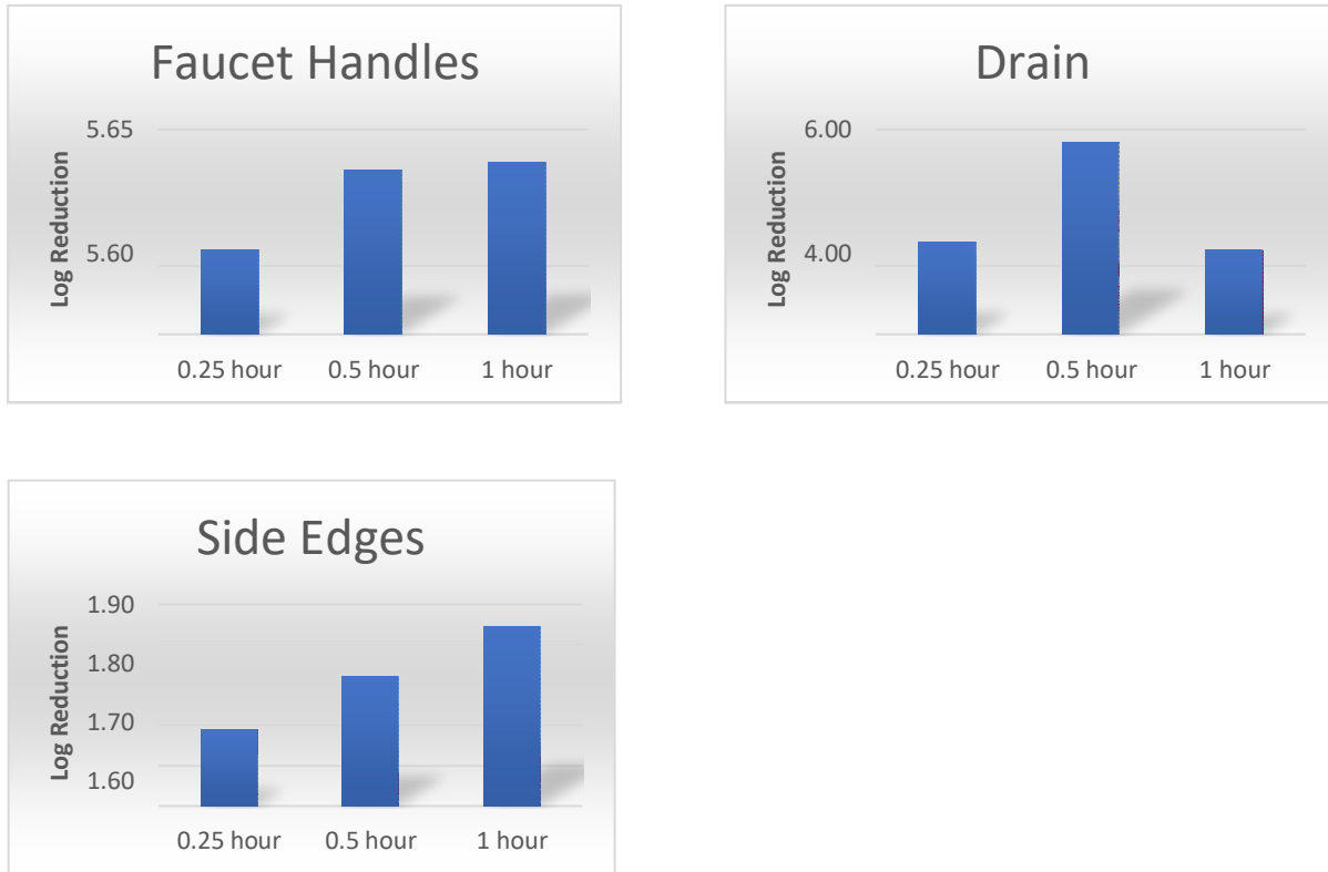
Figure 3: UV Reduction of E. coli Recovery on Vanity/Sink Surfaces
